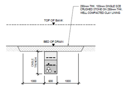
SECTION B SCALE 1:50
