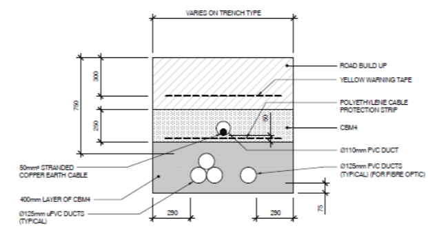
TYPICAL ROAD CROSSING DETAIL SCALE 1:20 [1 No. RADIAL]
