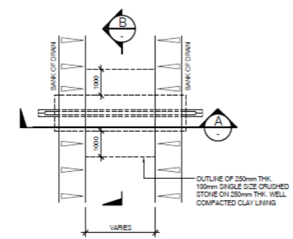
PLAN: TYPICAL TREFOIL FORMATION DRAIN CROSSING SCALE 1:100 [1 No. RADIAL]
