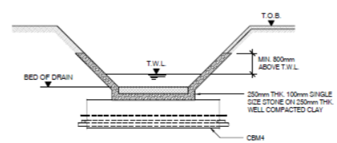
SECTION A SCALE 1:100
